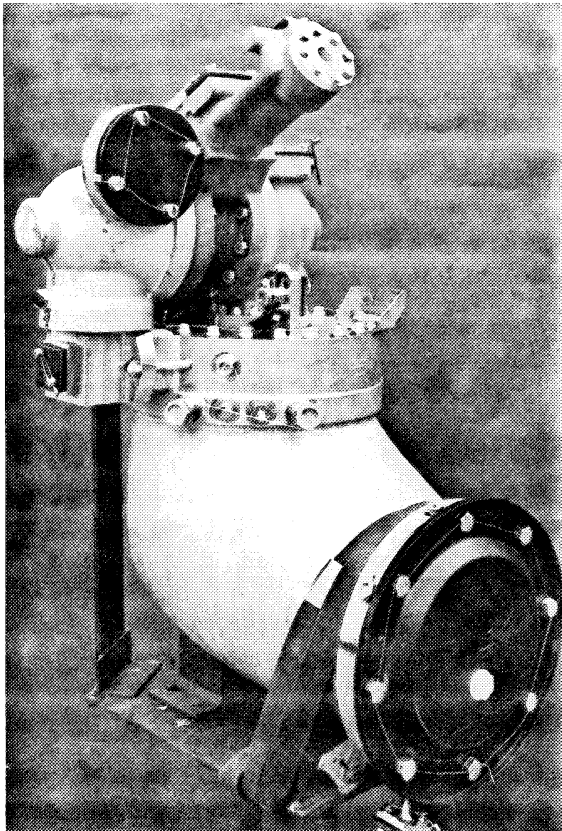
Gas Generator Assembly Including Control Valves
