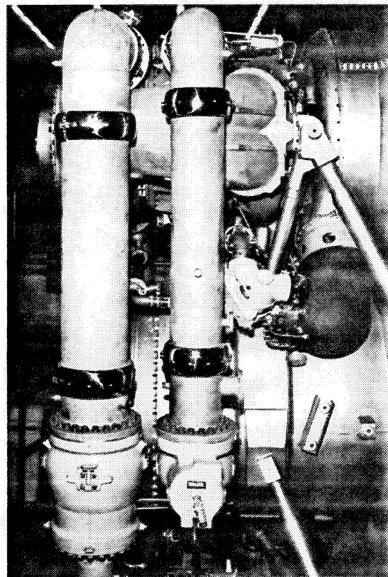
Propellant Feed—The main LOX valve and high-pressure line are shown at left. At right are the main fuel valve and high-pressure line.
